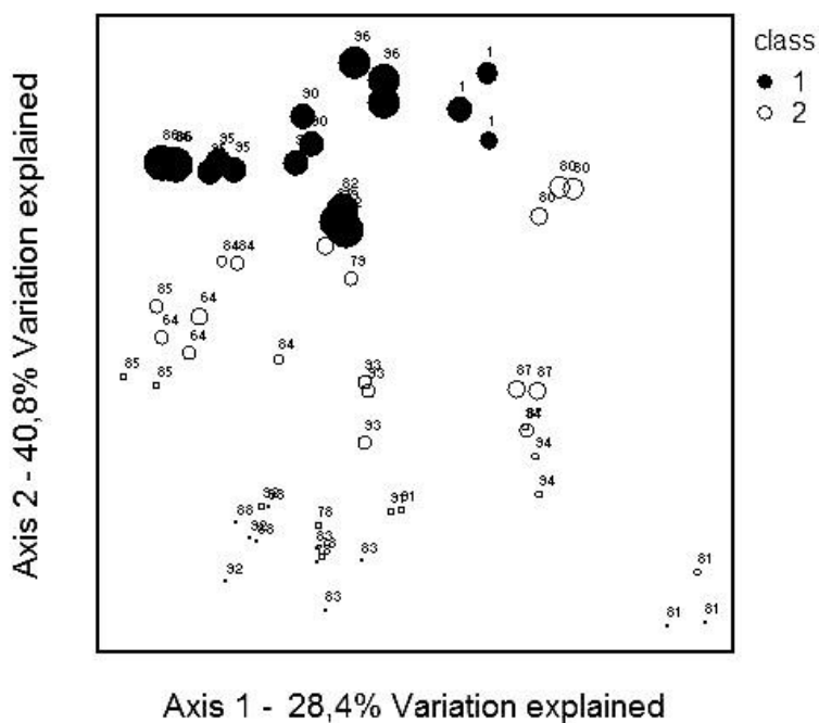
Figure 4. ISA indicator species ( Erica arborea ) in NMS analysis
