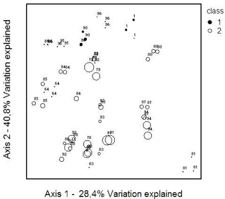
Figure 5. ISA indicator species ( Castanea sativa ) in NMS analysis
